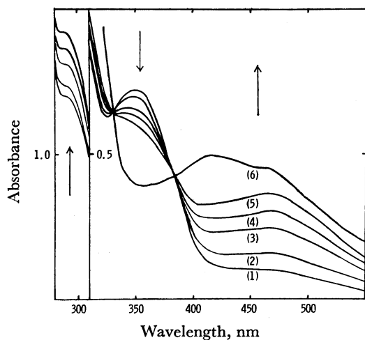
Fig. 4. Spectroscopic course of the reaction in o -BQDI- o -PD system in ethyl ether measured at room temperature. [o\text{-BQDI}] = 3.8 \times 10^{-3} M, estimated from the initial concentration of o -PD in the synthesis of o -BQDI, [o\text{-PD}] = 9.5 \times 10^{-4} M. (1) 1 min, (2) 8 min, (3) 41 min, (4) 85 min, (5) 164 min, (6) 24 hr after mixing.
