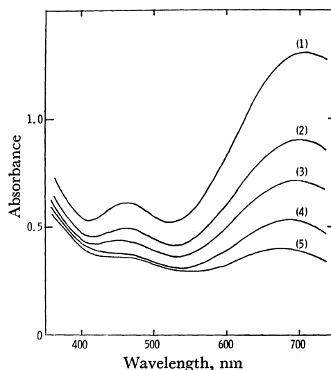
Fig. 1. The change of the outer complex bands with temperature in o -PD-CA system in ethyl ether. [\text{o-PD}] = 3.0 \times 10^{-3} M, [\text{CA}] = 1.5 \times 10^{-3} M. (1) -78^\circ\text{C} , (2) -72^\circ\text{C} , (3) -65^\circ\text{C} , (4) -55^\circ\text{C} , (5) -50^\circ\text{C} .
