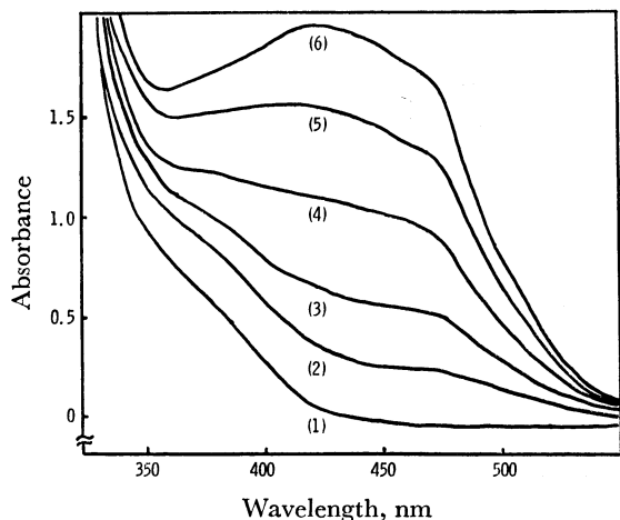
Fig. 3. Spectroscopic course of the reaction in o -PD-CA system in ethyl ether measured at room temperature. [o\text{-PD}] = 2.0 \times 10^{-3} M, [CA] = 1.0 \times 10^{-3} M. (1) 5 min, (2) 1 hr, (3) 2 hr 26 min, (4) 6 hr 13 min, (5) 13 hr 15 min, (6) 21 hr after mixing.
