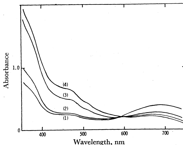
Fig. 2. Spectroscopic course of the reaction in o -PD-CA system in ethyl ether measured at several temperatures. [\text{o-PD}] = 3.0 \times 10^{-3} M, [\text{CA}] = 1.5 \times 10^{-3} M. (1) -44^\circ\text{C} , (2) -31^\circ\text{C} , (3) -20^\circ\text{C} , (4) -7^\circ\text{C} .
